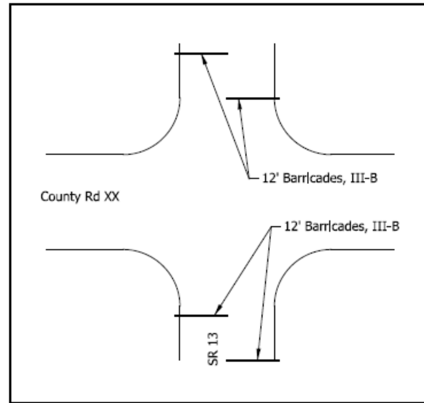
County Road Barricade Detail
